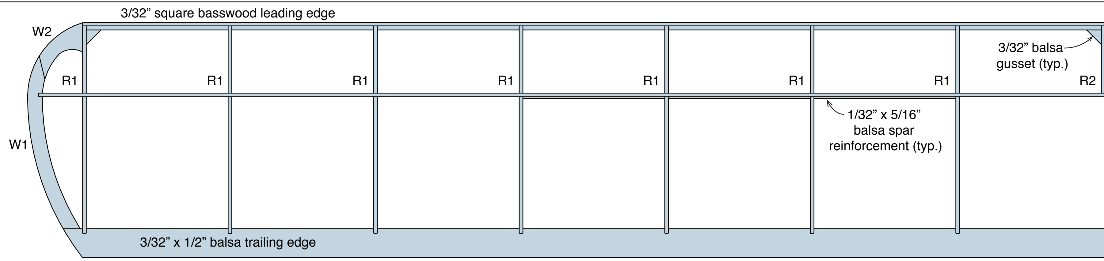
LEFT WING PLAN VIEW
