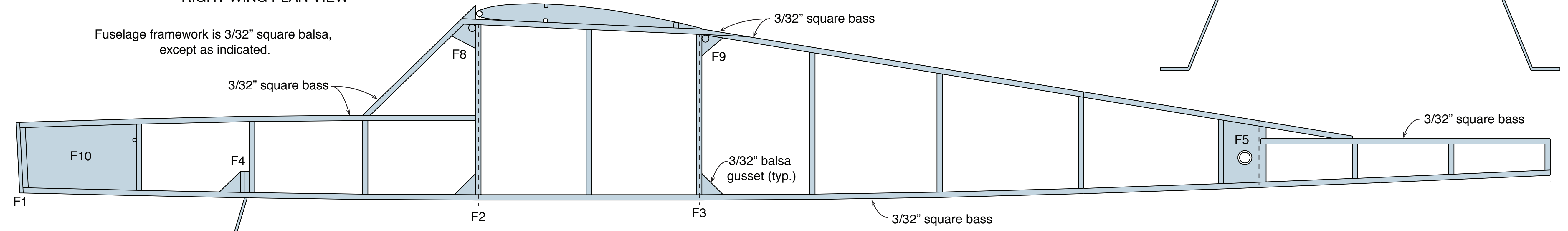
FUSELAGE SIDE ELEVATION
