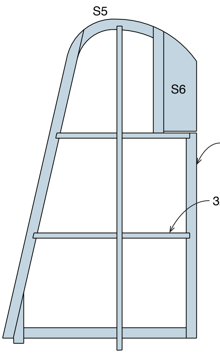
VERTICAL STABILIZER PLAN VIEW
